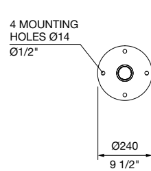
PLAN VIEW Baseplate
