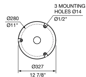
PLAN VIEW Cast Base
