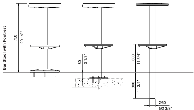
Cast Base Surface Fixed
