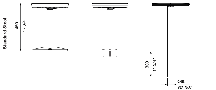
Cast Base Freestanding
